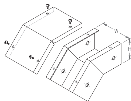
45 DEG. VERTICAL OUTSIDER RISER
