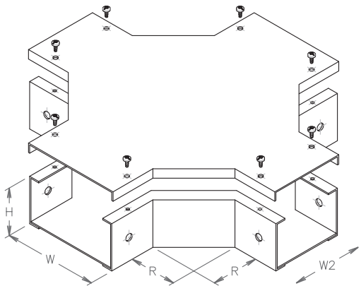
HORIZONTAL UNEQUAL CROSS
