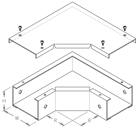
90 DEG. HORIZONTAL FLAT ELBOW
