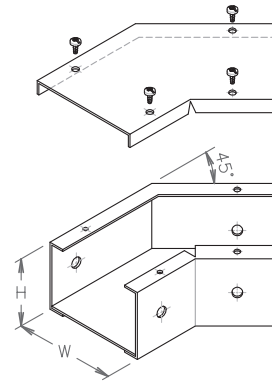
45 DEG. HORIZONTAL FLAT ELBOW
