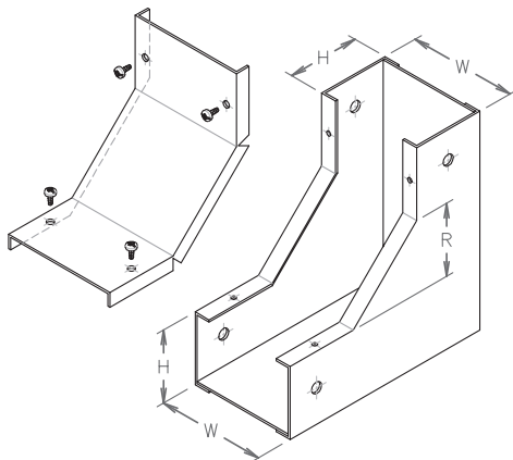
90 DEG. VERTICAL INSIDER RISER
