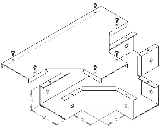
HORIZONTAL EQUAL TEE
