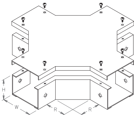
HORIZONTAL EQUAL CROSS
