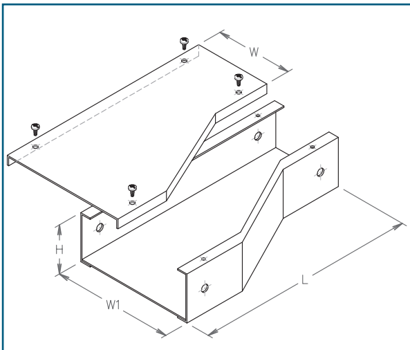
LEFT-HAND REDUCER
