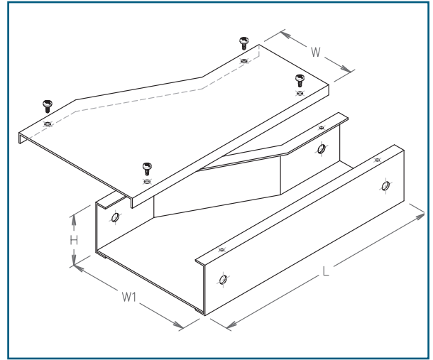
RIGHT-HAND REDUCER
