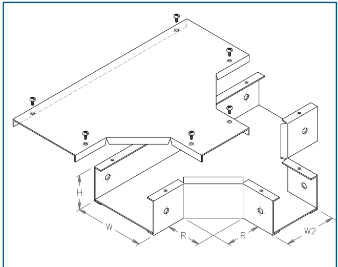
HORIZONTAL UNEQUAL TEE
