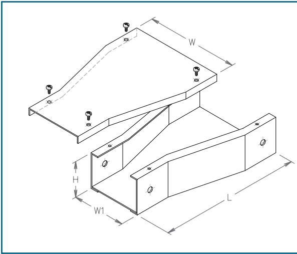
STRAIGHT REDUCER
