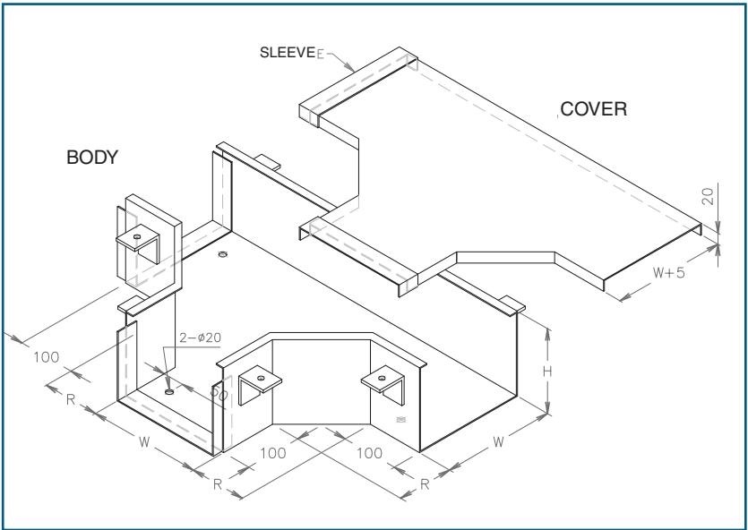
HORIZONTAL EQUAL TEE (W/O SEPARATOR)
