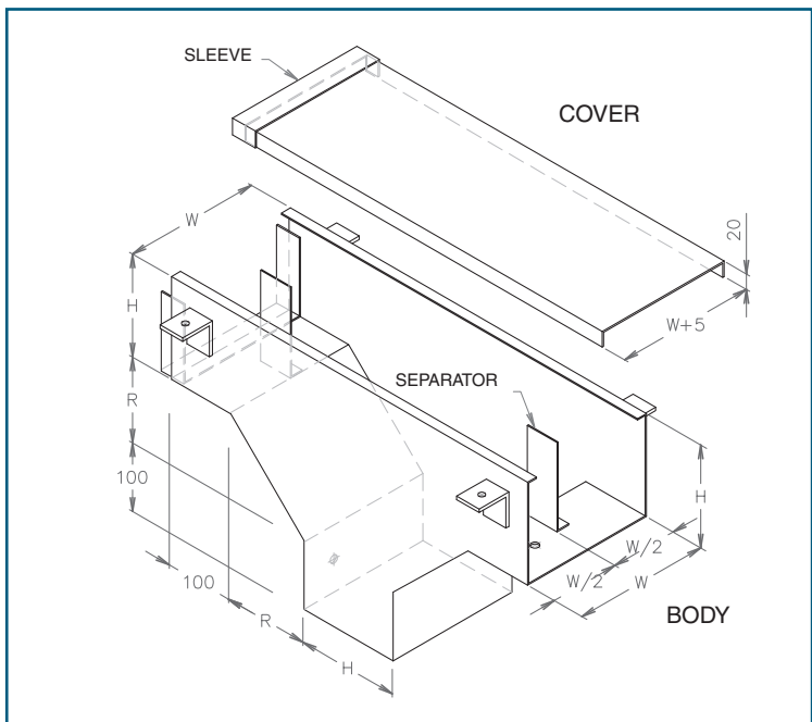
VERTICAL TEE (WITH SEPARATOR)
